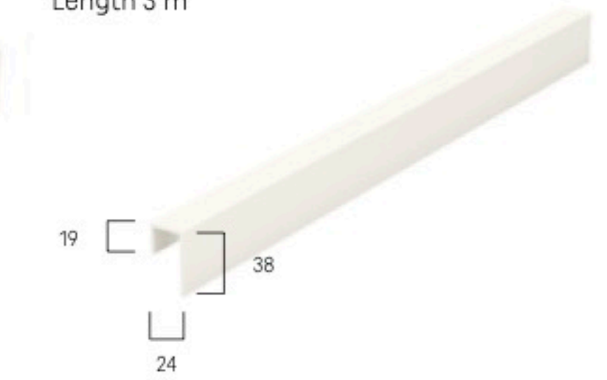
FS-262 Ventilation trim (two-part) Length 3 m
