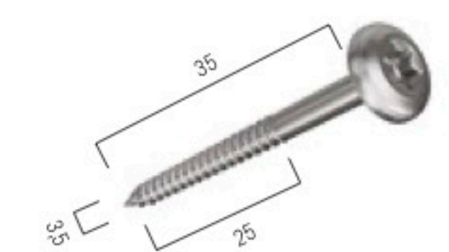
INOX-UP3.5X35-TX15-A2 Fitting screw
