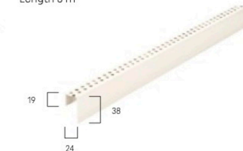
J-201 Joint cover for FS-201
